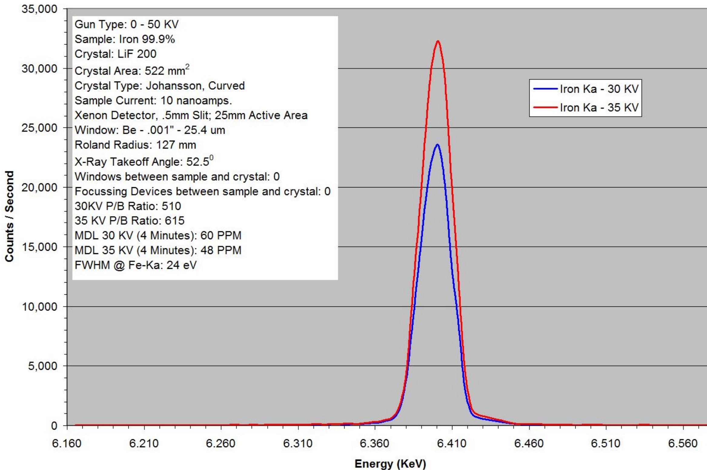
Figure 2: Iron Count Rate Performance with Xenon Detector
