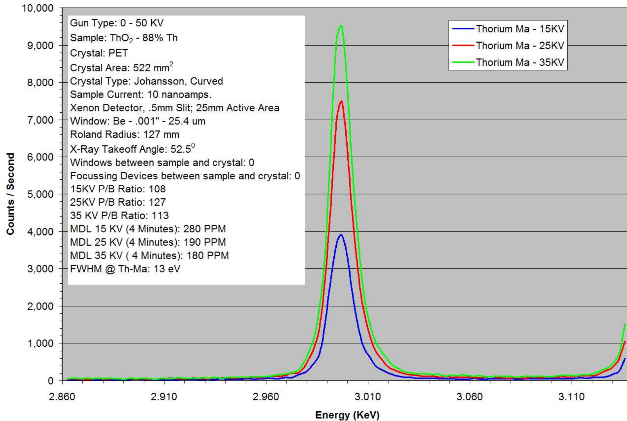
Figure 3: Thorium Count Rate Performance with Xenon Detector
