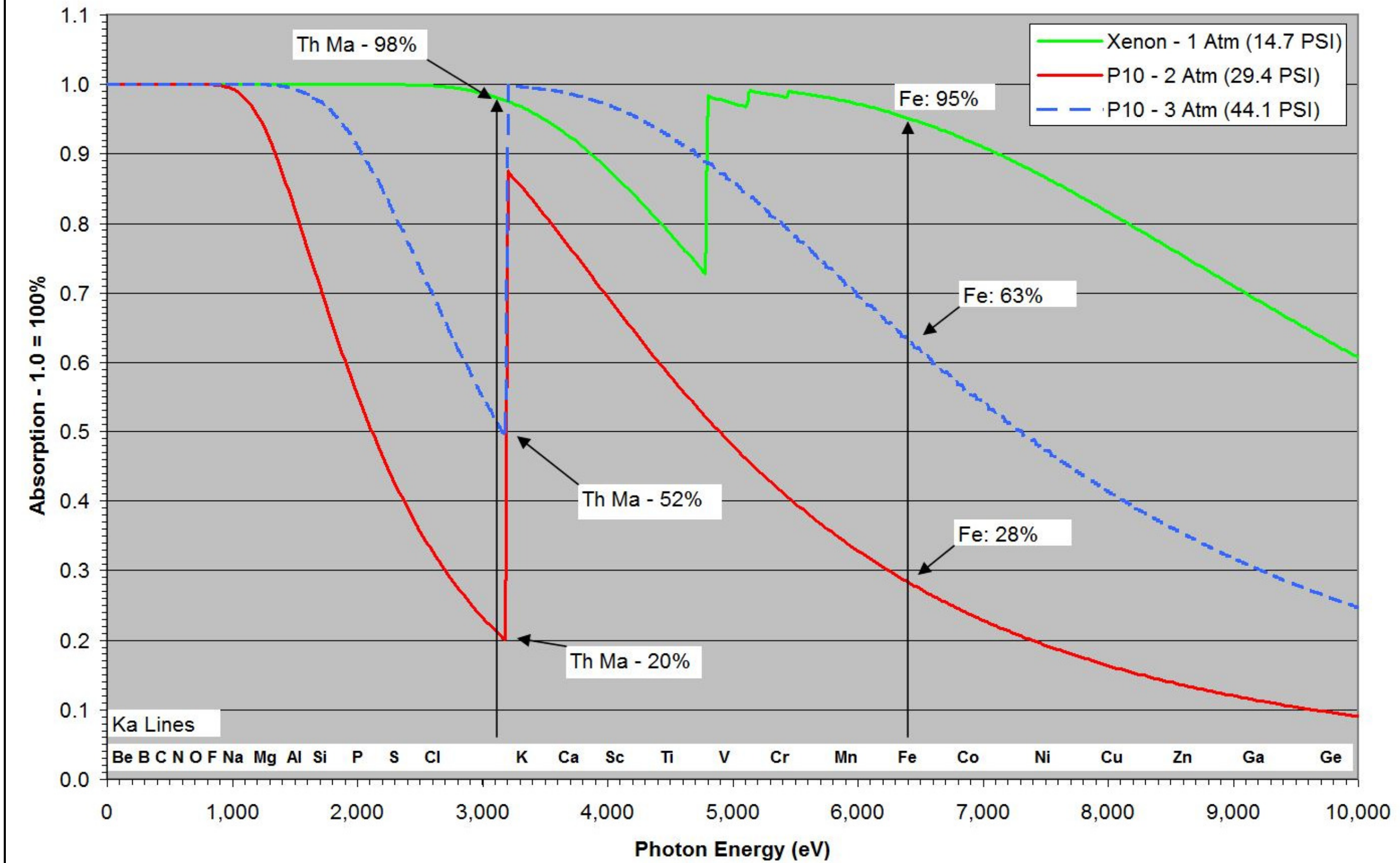
Figure 1: Advantages of Xenon Detector Gas
